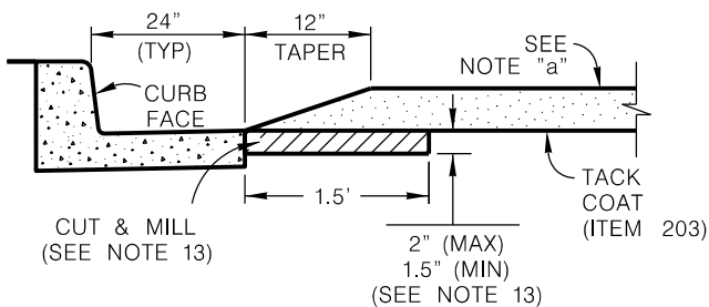
(CURB & GUTTER)
