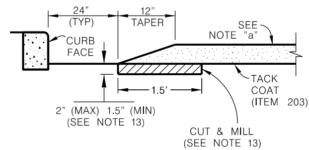
(STANDARD CURB)
