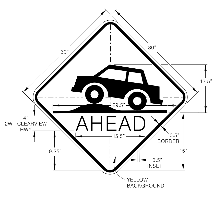
TRAFFIC SIGN DETAIL
